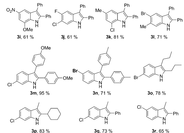
Scheme 3. Substrate scope. Reactions were carried out on a 0.3 mmol scale. Yields of isolated products are given.
