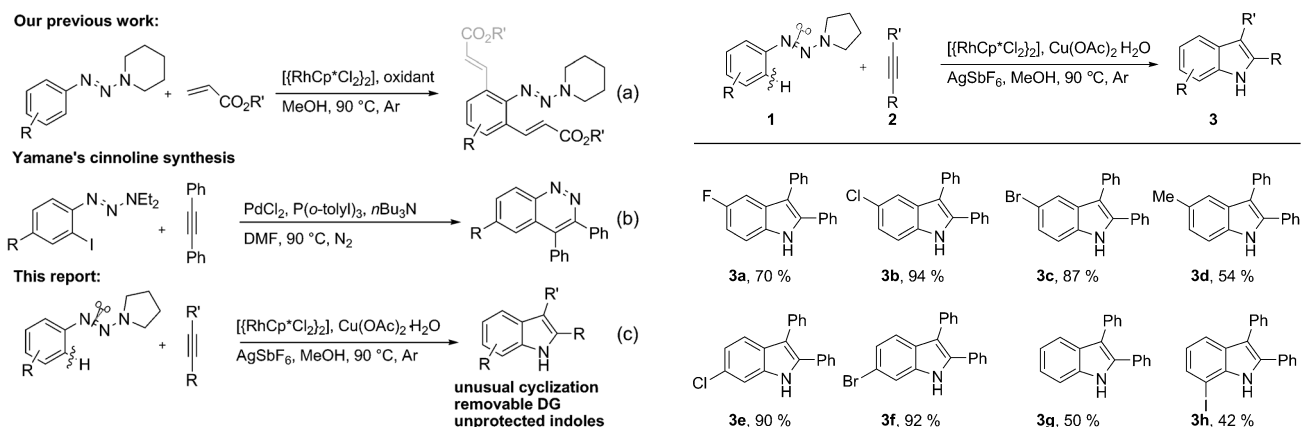
Scheme 2. Indole synthesis through triazene-directed C–H annulation. Cp* = pentamethylcyclopentadienyl.
